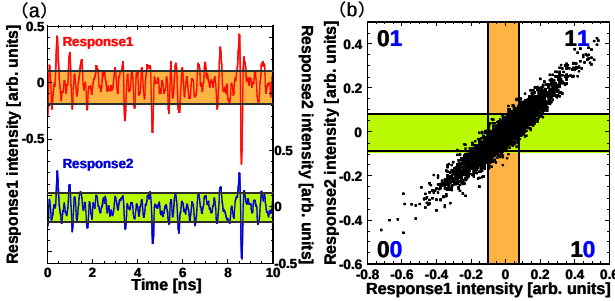
Fig. 6 Examples of the robust sampling method with two threshold values. (a) Temporal waveforms and (b) corresponding correlation plot. The two bits indicate Alice's and Bob's bits. 11 and 00 indicate that the same bit can be shared.
