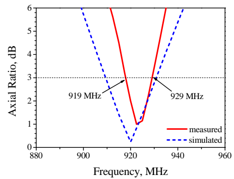
Figure 4: Measured and simulated axial ratio.
