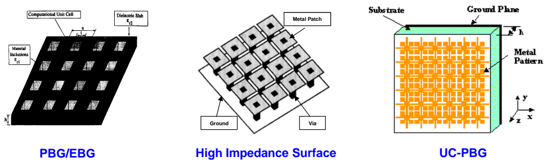
Fig. 7. Artificial Magnetic Ground Planes (AMGs). Synthesized 2-D or 3-D periodic metallic or dielectric structures to effectively impede the propagation of electromagnetic waves in a specified band of frequency.
