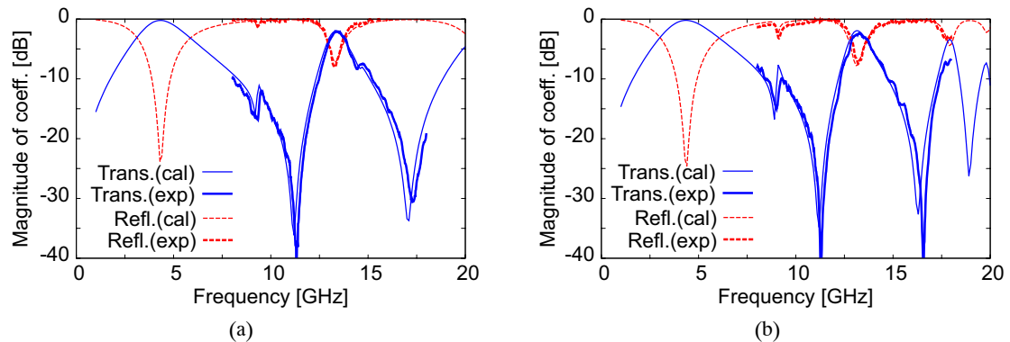
Fig. 6. Comparison of the frequency characteristics between the calculated and the measured results of the gridded eight-legged elements.
