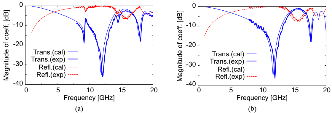
Fig. 5. Comparison of the frequency characteristics between the calculated and the measured results of the FSS with eight-legged element.
