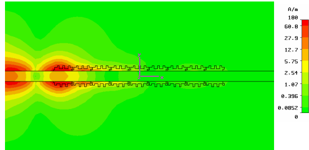
(b) Interdigital-mushroom ( f_0 = 4.01\text{GHz} )
