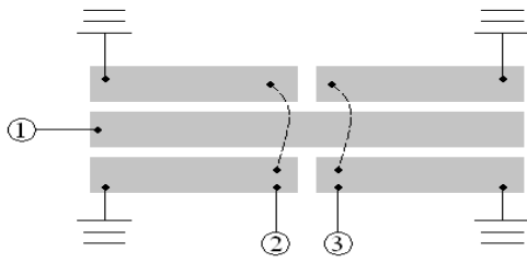
Fig. 2 Parallel coupled lines balun
