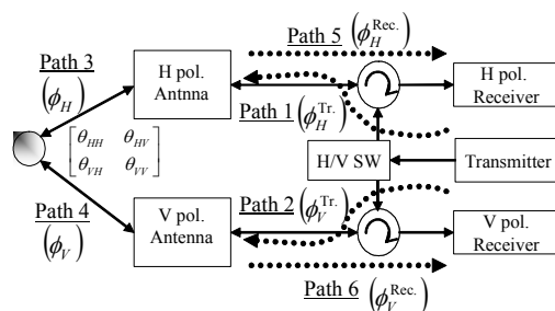
Fig.1 System block diagram of polarimetric imaging radar.
