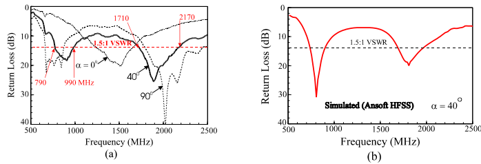
Figure 3. (a) Measured and (b) simulated return loss for the proposed antenna with various values of \alpha = 40^\circ .
