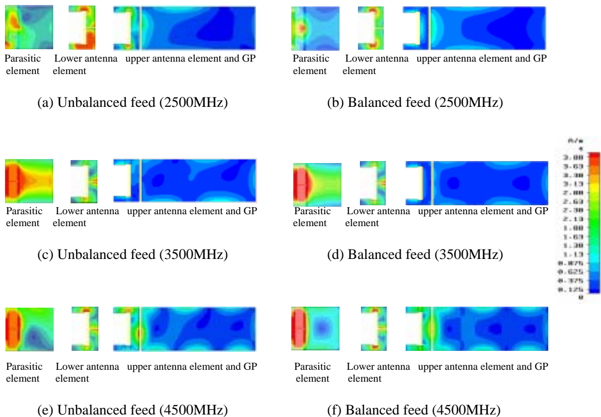
Fig.4 Current distribution
