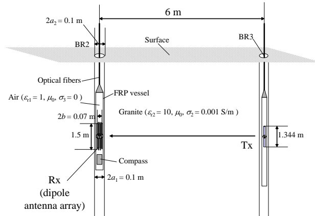
Fig. 4. Experiment to transmit a wave to the dipole array in granite from outside the borehole in O.E.C.U., Shijonawate, Japan.
