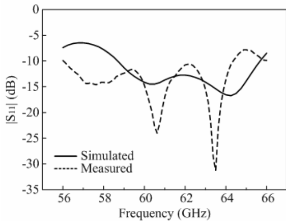
Fig. 4: Measured and simulated and input return losses of the 1×4 sequentially-rotated prototype antenna.
