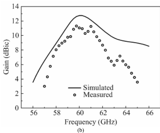
Fig. 5: Measured and simulated (a) axial ratios and (b) RHCP peak gains of the 1×4 sequentially-rotated prototype antenna.
