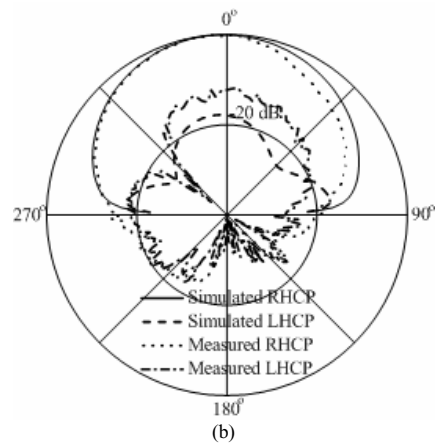
Fig. 6: Measured and simulated radiation patterns of the 1×4 sequentially-rotated prototype antenna. (a) x-z and (b) y-z plane patterns.
