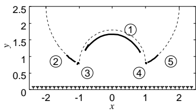
Fig. 4. Estimated target shape using SEABED.
