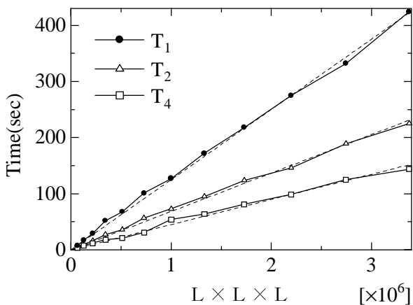
Fig.5 The computation time (Our method)
