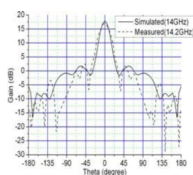
(e) H-plane pattern without HIS
