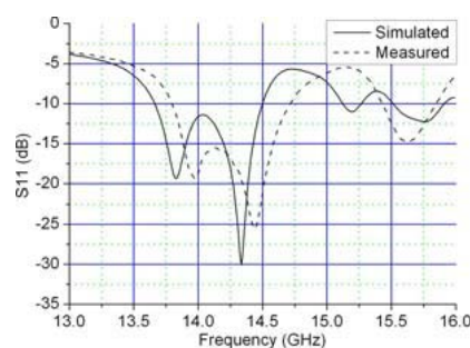
(b) Returned loss for the case with HIS
