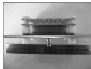
(b) Prototype fed by U-slotted patch
