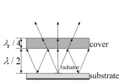
Figure 1 Structure of Fabry-Perot antenna
