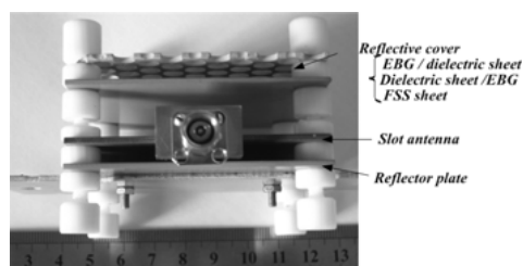
(a) Prototype fed by wide-slot
