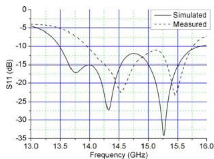
(a) Returned loss for the case without HIS
