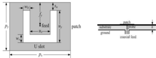
(a) Top view (b) Front view Figure 3 Structure of U-slotted rectangular patch radiator
