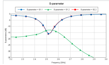
Fig. 3. S-parameter of the MIMO system.
