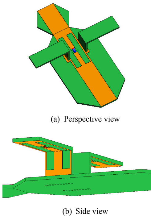
Fig. 1. Coupler applied military-use small platform
