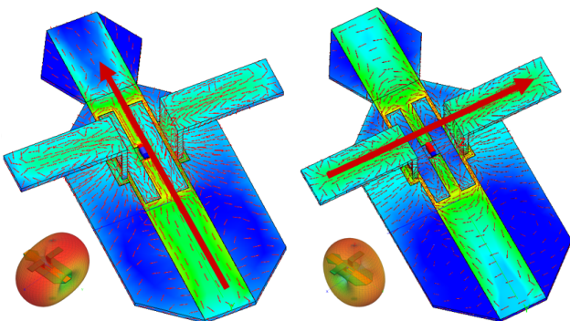
Fig. 2. Current distribution and radiating pattern of each radiating modes (Left: mode 1, Right: mode 2)
