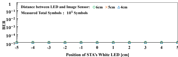
Fig. 5. BERs versus Position of Single LED or 16-element LED Array in the Station.
