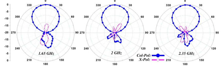
Fig. 3 Radiation patterns
