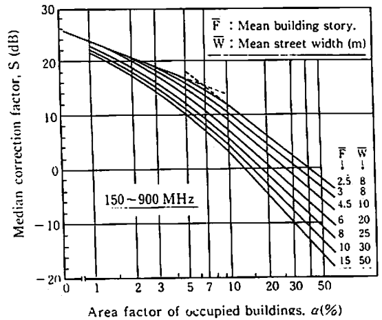
Fig. 4 Prediction curves of median correction factor, S , as a function of a , \bar{F} and \bar{W}
