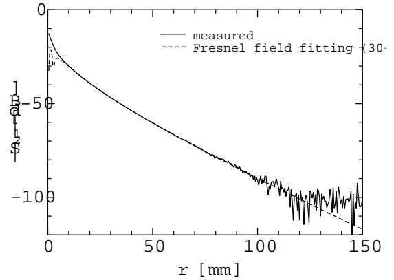
Fig. 6: Measured |S_{21}| and its curve fitting based on the Friis transmission formula in the near-field region.
