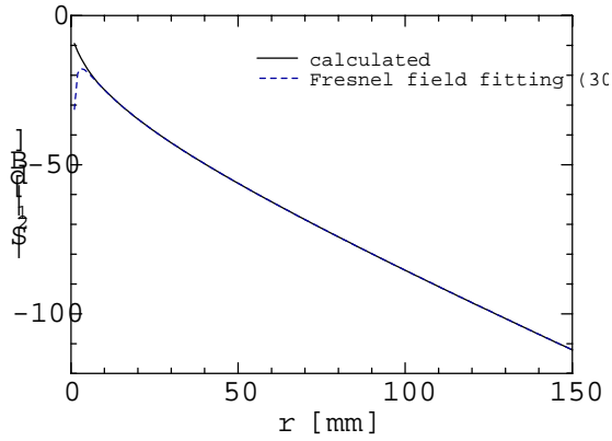
Fig. 4: Calculated |S_{21}| and its curve fitting based on the Friis transmission formula in the near-field region.
