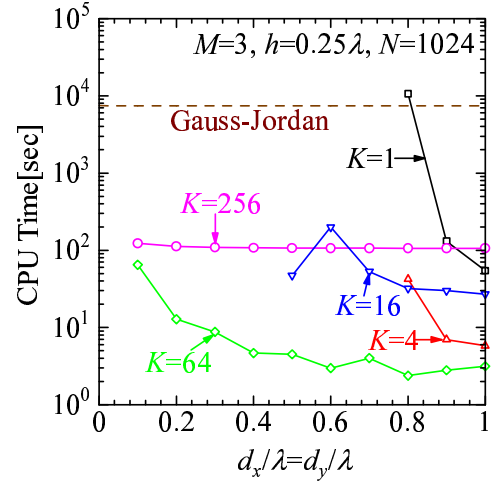
Figure 4: CPU time versus array spacing.
