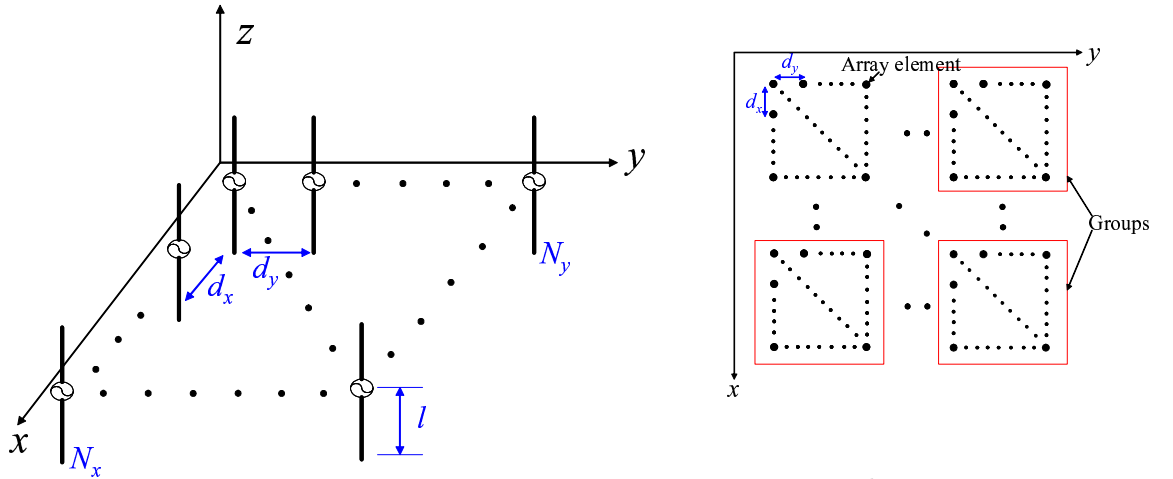
Figure 2: Each group contains several neighbouring array elements.
