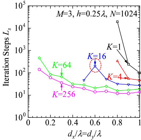
Figure 3: Required iteration steps versus array spacing.
