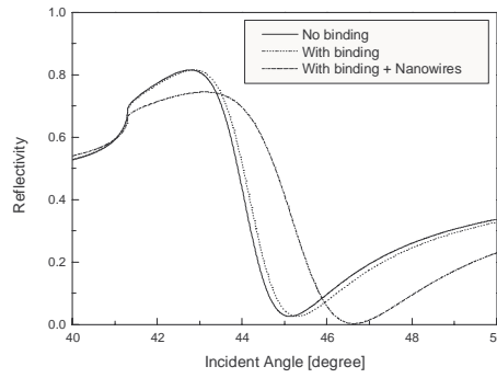
Figure 2. SPR curves (reflectivity vs. incident angle) of a 40 nm thick Au metal film on a dielectric glass prism (solid line), binding with biomaterial on a bare Au film (dotted line), and the nanowire layer is additionally adsorbed onto biomaterial layer (dashed line). In the calculation, the period of nanowire gratings is 400 nm. The calculated resonance angles are 45.125° (solid line), 45.295° (dotted line), and 46.460° (dashed line), respectively.
