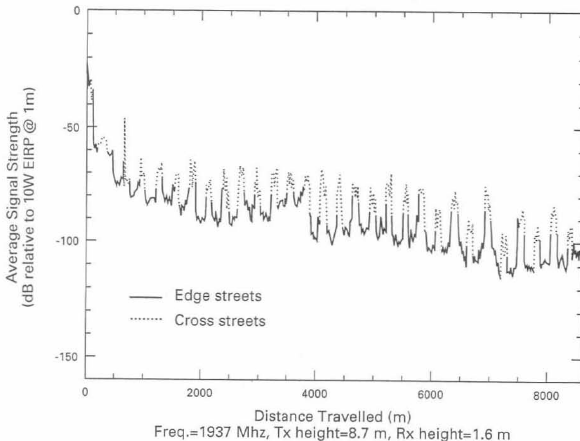
Fig. 2. Received Signal Strength along a zig-zag path in the Sunset District.
