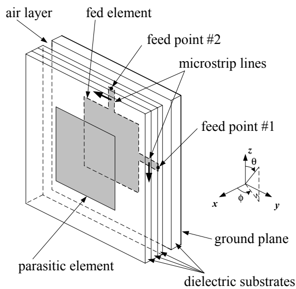
Fig.4 Configuration of a dual-polarized square patch antenna with a parasitic element
