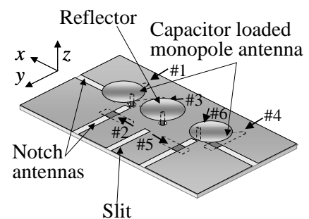
Fig. 1 Proposed antenna.
