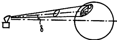
Fig. 1 The antenna with elliptical beam cross-section.
