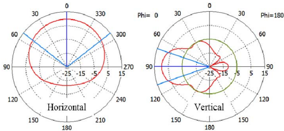
Fig.4 Radiation pattern with FSS
