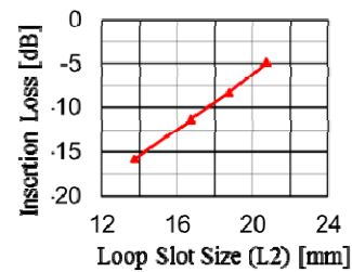
Fig.2 Insertion loss property
