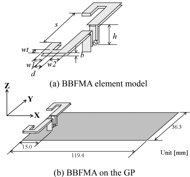
Fig.1 Configuration of BBFMA ( w1=w2=d=5 , wt=1.5 , b=0.5 , h=7 , s=24 [mm])
