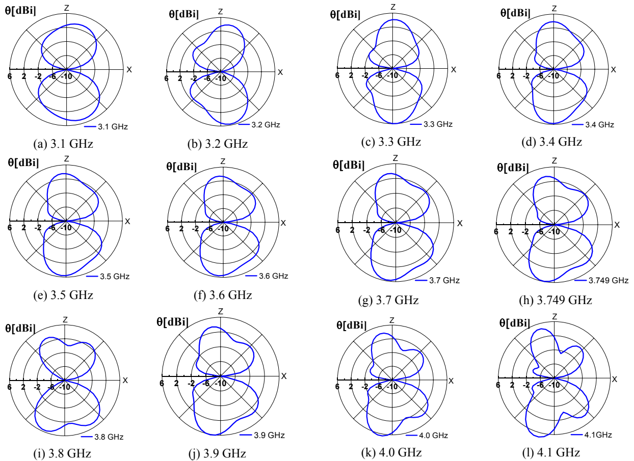
Figure 3. The electric field radiation characteristics B = 60 mm, W1 = 1.2 mm, W2 = 2.4 mm, L1 = 11.2 mm, L2 = 10.5 mm, ws = 2.4 mm, g = 0.2 mm, U = 10 mm
