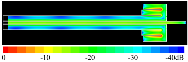
Figure 7 Current distribution at 3.824 GHz B = 60 mm, W1 = 1.2 mm, W2 = 2.4 mm, L1 = 11.2 mm, L2 = 10.5 mm, ws = 3.6 mm, g = 0.2 mm, U = 8.8 mm
