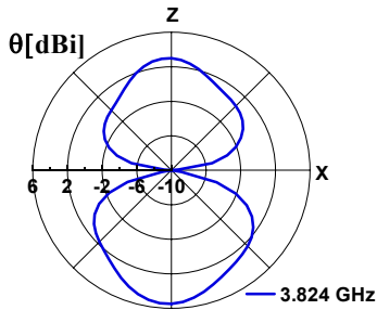
Figure 8 Electric field radiation characteristics at 3.824 GHz B = 60 mm, W1 = 1.2 mm, W2 = 2.4 mm, L1 = 11.2 mm, L2 = 10.5 mm, ws = 2.4 mm, g = 0.2 mm, U = 8.8 mm
