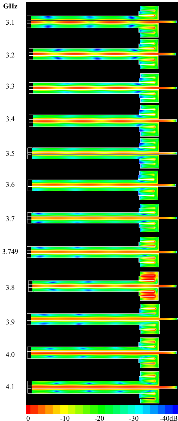
Figure 2 Current amplitude distribution B = 60 mm, W_1 = 1.2 mm, W_2 = 2.4 mm, L_1 = 11.2 mm, L_2 = 10.5 mm, w_s = 2.4 mm, g = 0.2 mm, U = 10 mm
