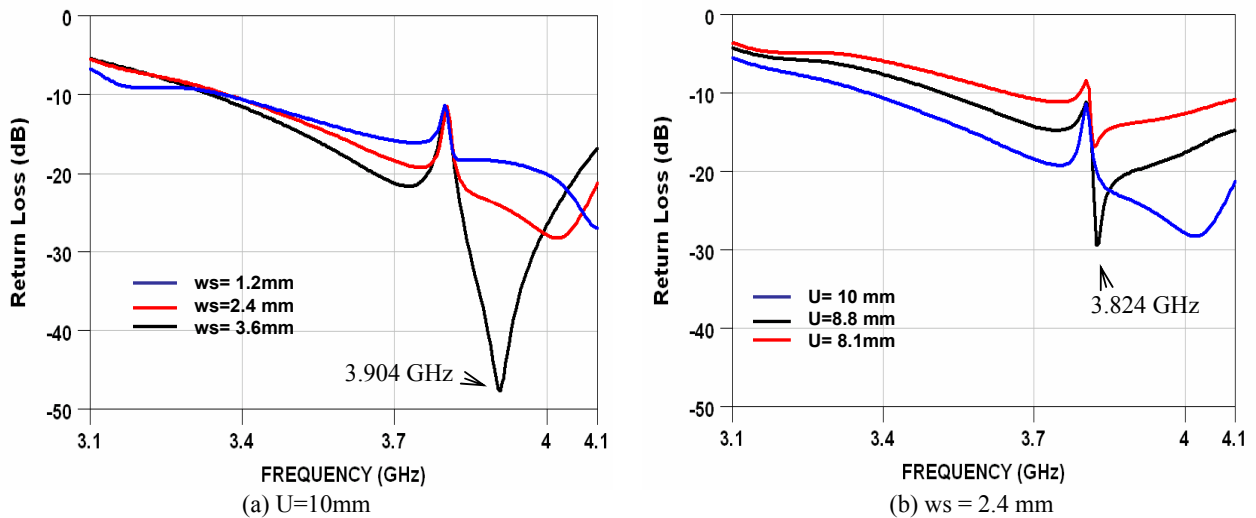
Figure 4. Return loss characteristics. B = 60 mm, W1 = 1.2 mm, W2 = 2.4 mm, g = 0.2 mm
