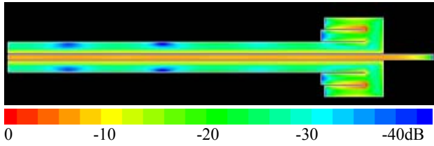
Figure 5 Current distribution at 3.904 GHz B = 60 mm, W1 = 1.2 mm, W2 = 2.4 mm, L1 = 11.2 mm, L2 = 10.5 mm, ws = 3.6 mm, g = 0.2 mm, U = 10 mm
