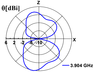
Figure 6 Electric field radiation characteristics at 3.904 GHz B = 60 mm, W1 = 1.2 mm, W2 = 2.4 mm, L1 = 11.2 mm, L2 = 10.5 mm, ws = 3.6 mm, g = 0.2 mm, U = 10 mm.
