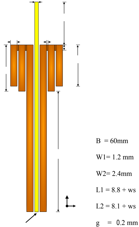
Figure 1 Structure of planar sleeve antenna
