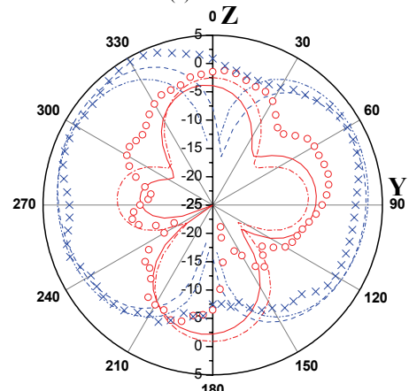
(c) 4.5GHz
