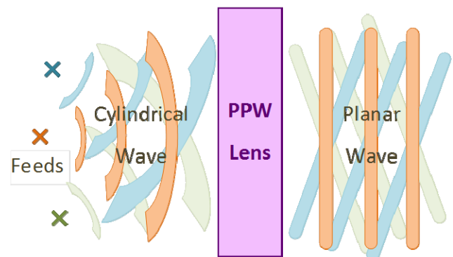
Fig. 1. Principle of operation of the lens.
