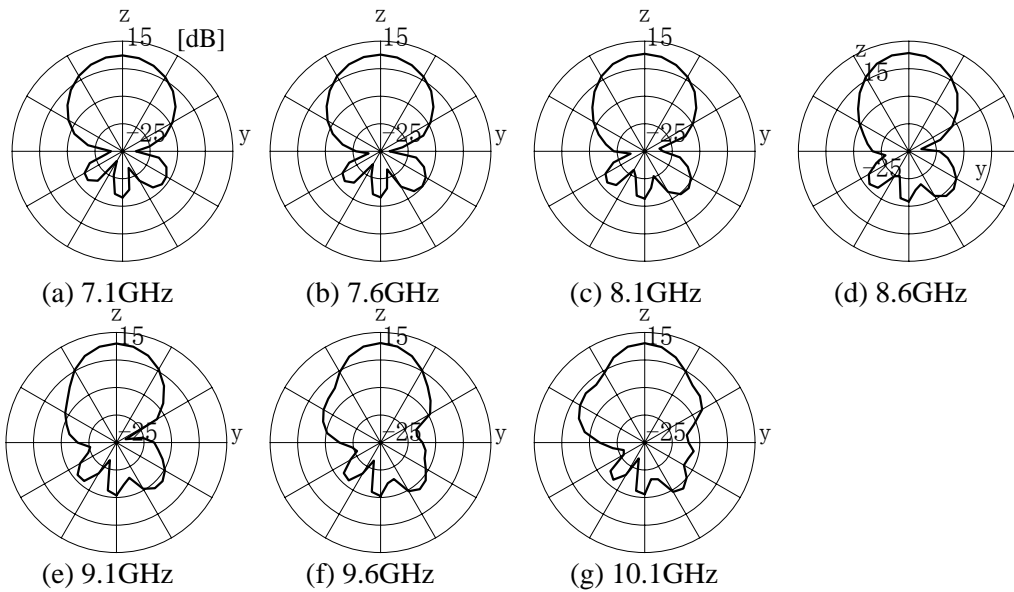
Figure 7: Electric field radiation patterns of antenna Model 2 in yz plane.
