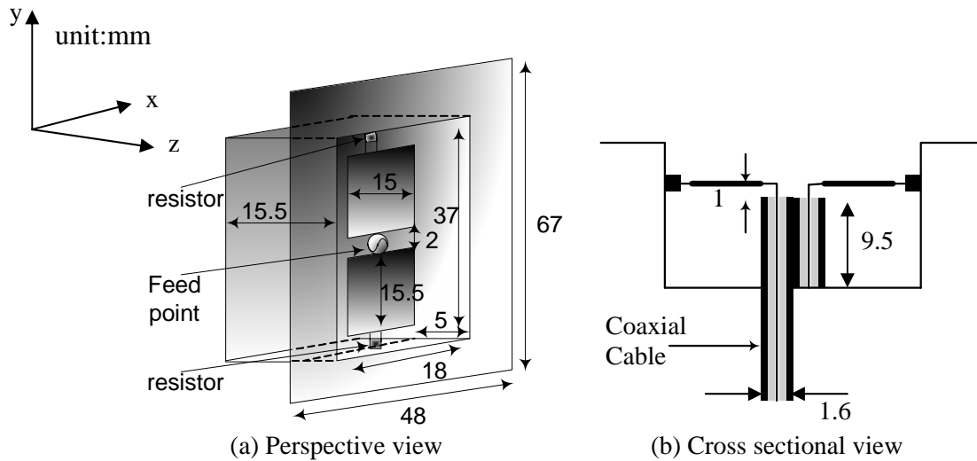
Figure 1: Structure of antenna Model 1.
