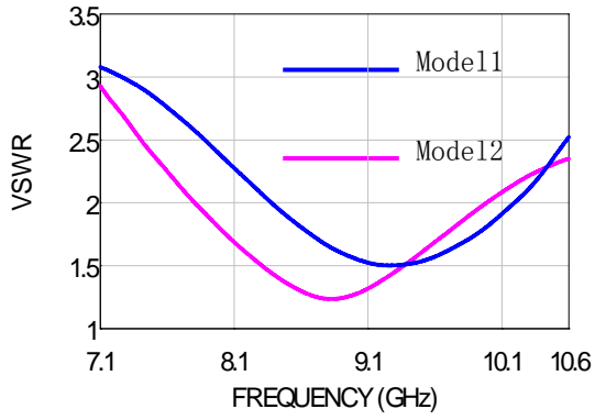
Figure 3: VSWR characteristics.
