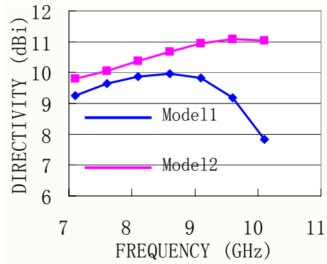
Figure 4: Directivity of two antennas.
