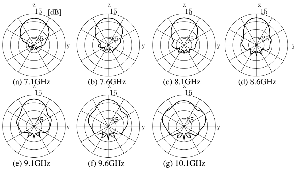
Figure 5: Electric field radiation patterns of antenna Model 1 in yz plane
