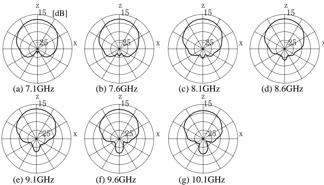
Figure 6: Electric field radiation patterns of antenna Model 1 in xz plane
