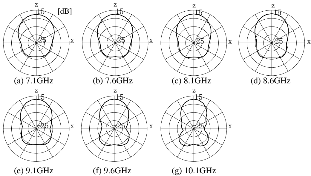
Figure 8: Electric field radiation patterns of antenna Model 2 in xz plane.
