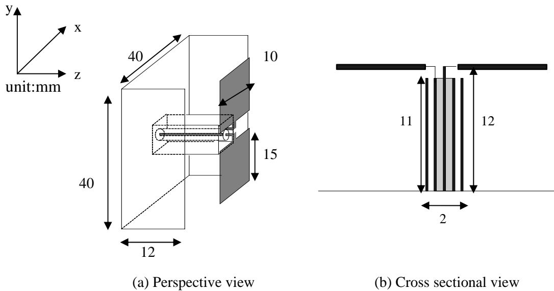
Figure 2: Structure of antenna Model 2.
