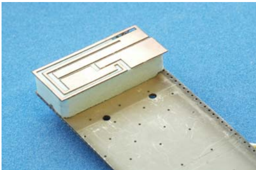
Figure 2: Quadband patch antenna for mobile telephones(IMST, [2])
