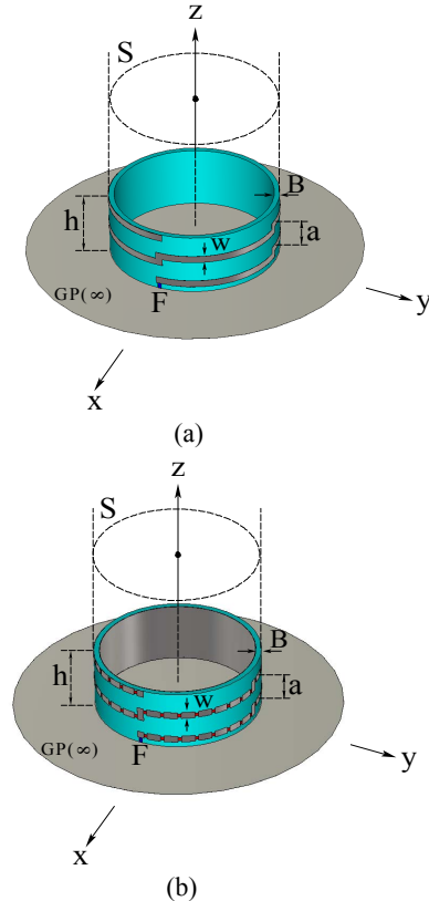
Figure 1: Helical antennas. (a) Conventional helical antenna. (b) Novel helical antenna.
