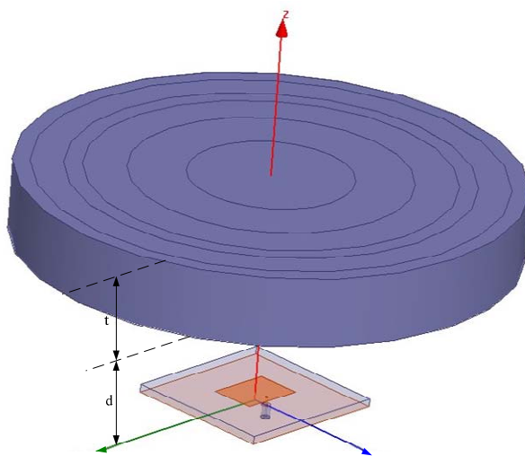
Figure 1. The structure of the plane lens antenna
