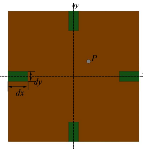
Fig.3. geometry of proposed antenna (a)the patch element ( \rho = 0.35 ) (b) top view and the side view (P is the feed point) (c) view from the ground-plane side
