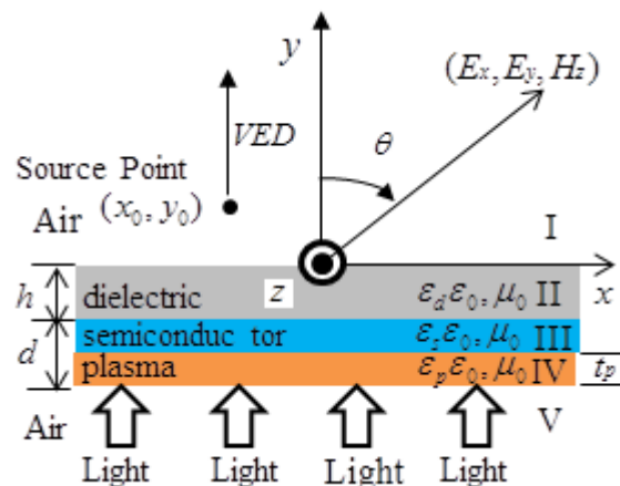
Fig. 1. Geometry of a vertical electric dipole above a dielectric slab backed by a photonically plasma-induced semiconductor slab
