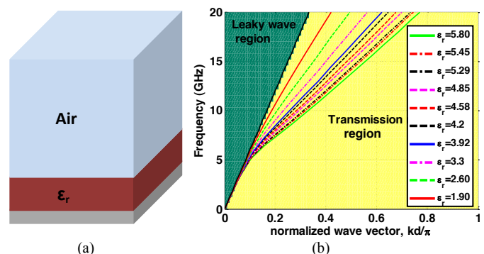
Fig. 1. (a) A sketch of the unit cell for which the dispersion curve has been numerically calculated (b) The dispersion curves for numerous values of relative permittivity.
