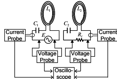
Fig. 4 Measurement setup by oscilloscope
