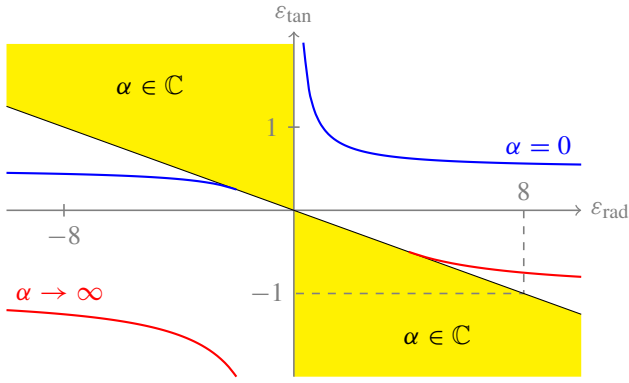
Fig. 1. The polarizability of an ideal RU sphere is well defined in the first and third quadrants of the \epsilon_{\text{rad}} \epsilon_{\text{tan}} -plane. The potential at the origin is singular if \epsilon_{\text{rad}} and \epsilon_{\text{tan}} have opposite signs, and in the yellow regions the potential and polarizability are complex. Also shown are the lines where the polarizability vanishes (blue lines in the upper half-plane) and where the polarizability is singular (red lines in the lower half-plane).
