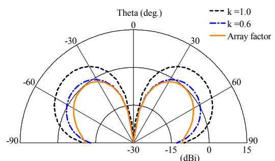
(b) Cross-polarization
