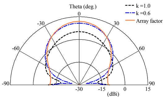
(a) Co-polarization
