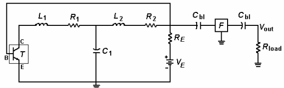
Figure 2. Chaotic oscillator
