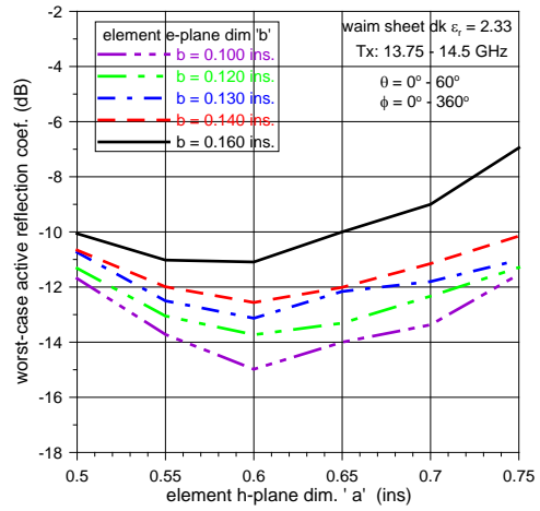
Fig. 8 Worst-case match within Tx band, dk=2.33
