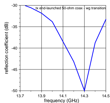
Fig. 13 Transition match at Tx band.
