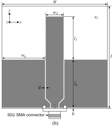
Fig. 4: Structures of the designed antennas. (a) Monopole antenna with a 1-D EBG cell (b) Reference conventional monopole antenna
