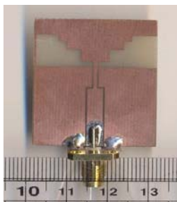
Fig. 2: Implemented Antenna
