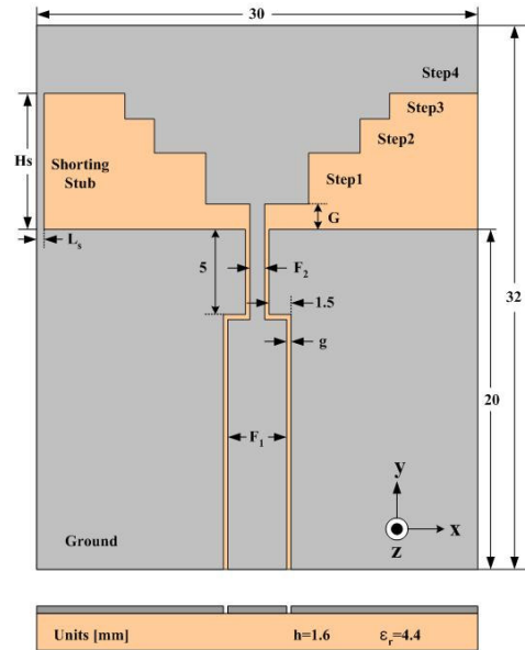
Fig. 1: Geometry of the proposed CPW-Fed ground short-circuited staircase rectangular monopole UWB antenna
