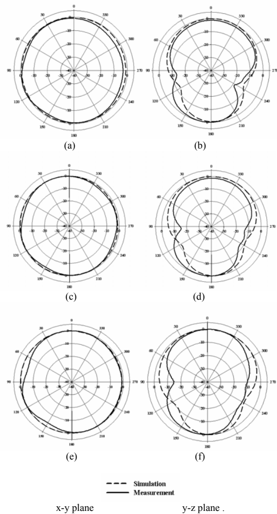
Fig. 3. Simulated and Measured radiation patterns (a) E-plane of 1.7 GHz (b) H-plane of 1.7 GHz (c) E-plane of 1.8 GHz (d) H-plane of 1.8 GHz (e) E-plane of 1.9 GHz (f) H-plane of 1.9 GHz
