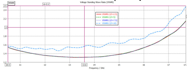
Fig. 3. The VSWR of different feeding positions.
