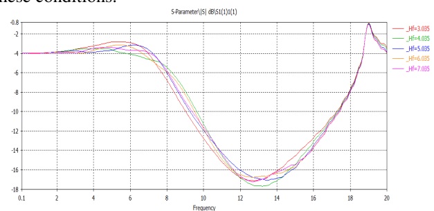
Fig. 6. The reflection coefficients VS. length of the probe.
