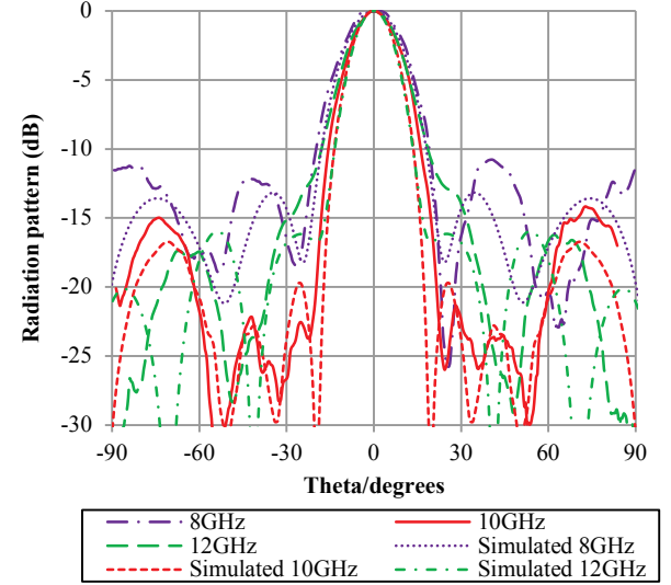
Fig. 3. Far-field radiation patterns of the 3D-printed FL in H-plane at different frequencies
