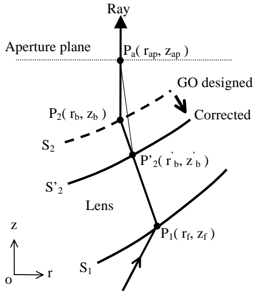
Fig.5 Phase correction by lens shaping
