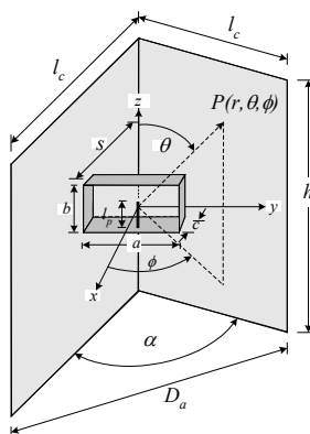
Fig. 1 Antenna structure.
