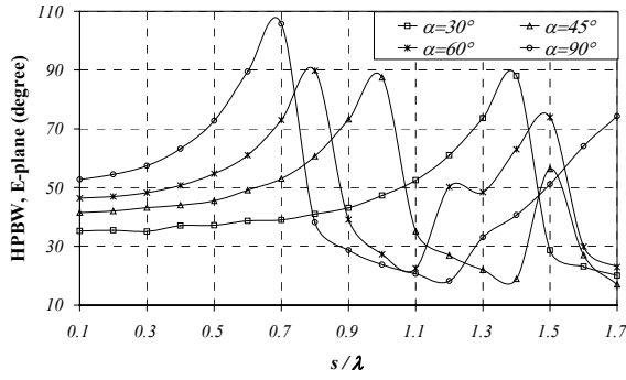
(a) Half power beamwidth (E-plane)
