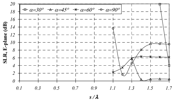
(a) Side lobe ratio (E-plane)
