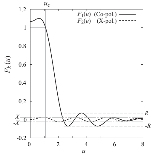
Fig. 1. Parameters for quadratic programming.
